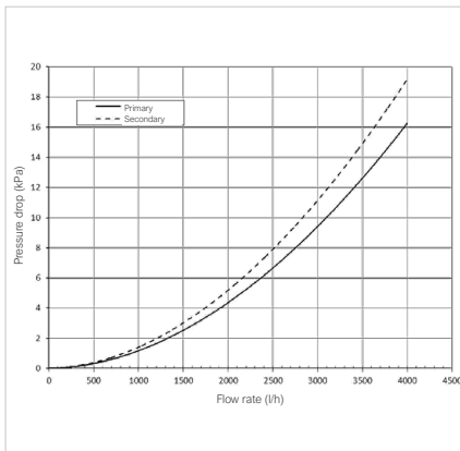
Separation plate heat exchanger Pressure drop
